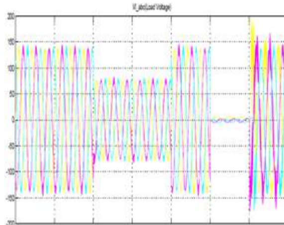
Voltage sag due to 3-phase fault without DVR
